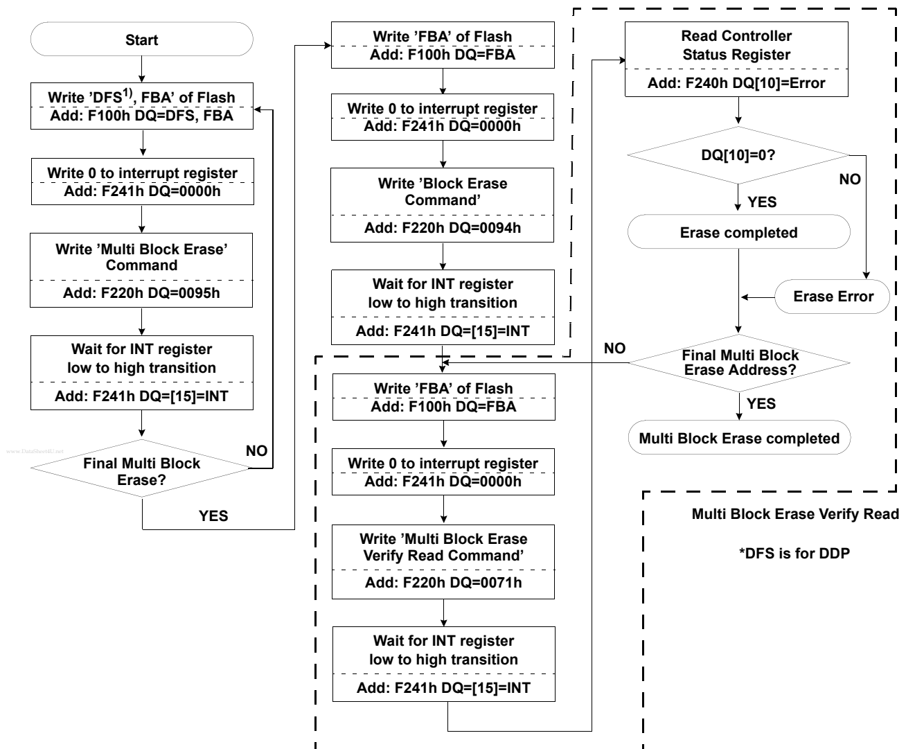
Multi Block Erase/ Multi Block Erase Verify Read Flow Chart
