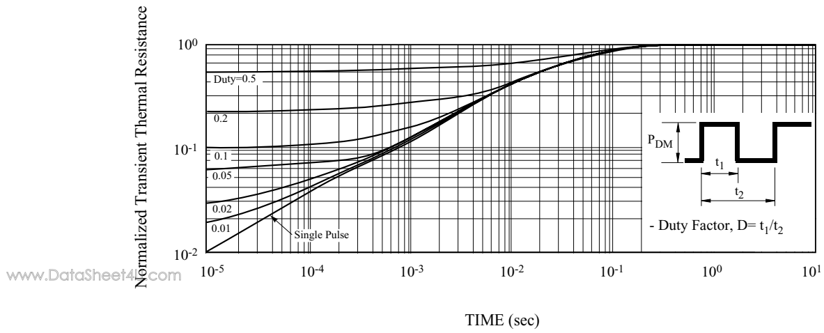
Fig12. Transient Thermal Response Curve
