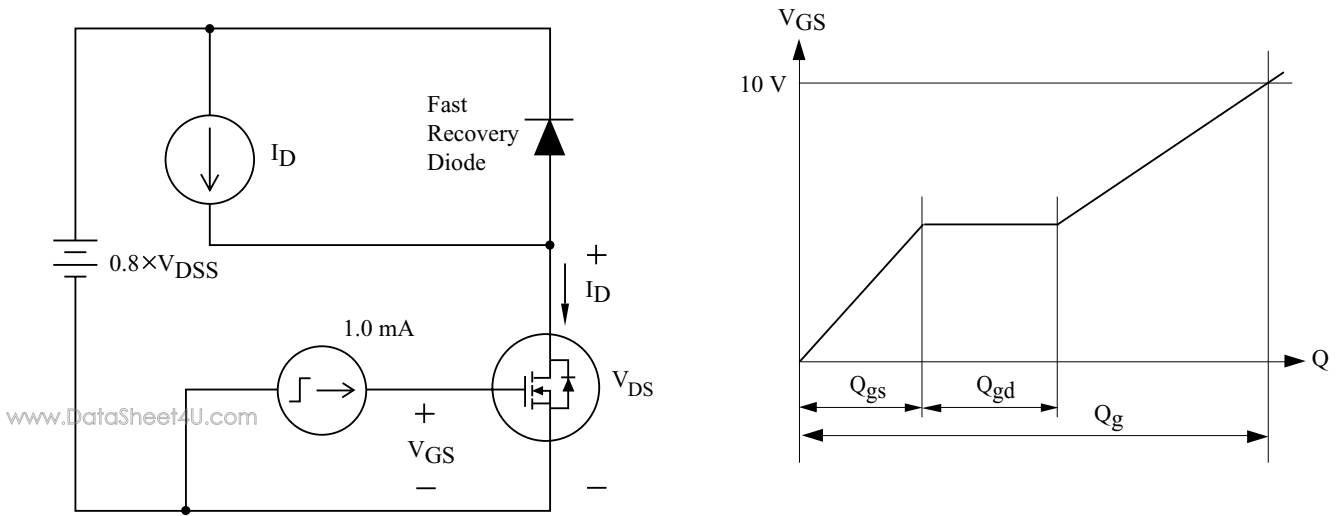
Fig14. Gate Charge
