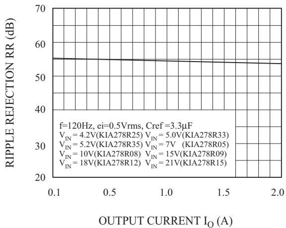
Fig.20 I_O - RR
