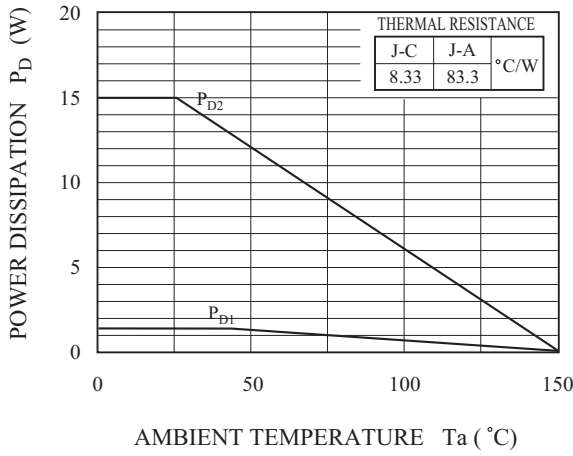
Fig.4 P_D - T_a
