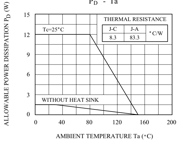
P_D - T_a
