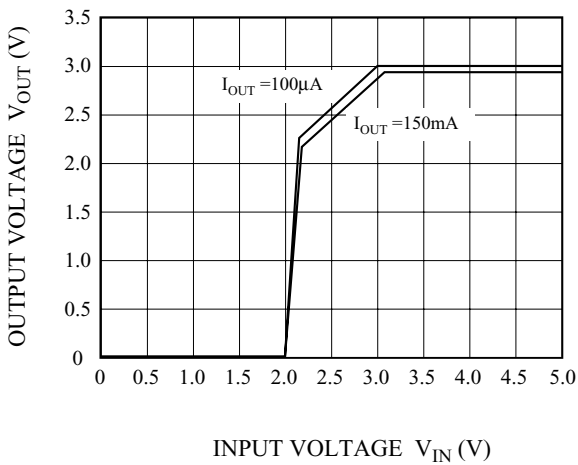
Fig. 3 V IN - V OUT
