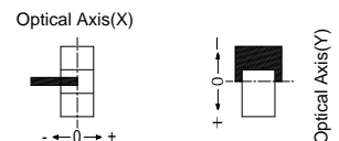
Method of measuring position detection characteristic
