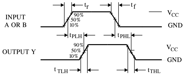
Figure 1. Switching Waveforms
