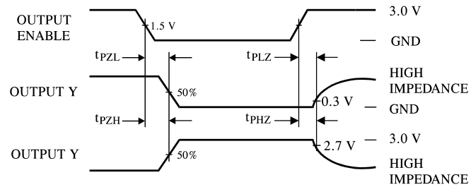
Figure 3. Switching Waveforms
