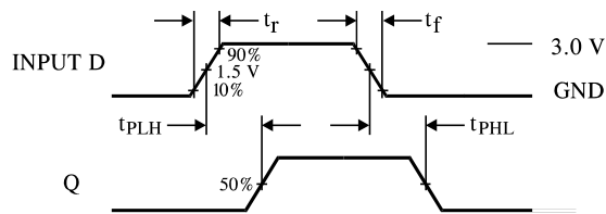
Figure 1. Switching Waveforms
