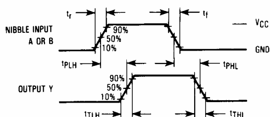
Figure 1. Switching Waveforms
