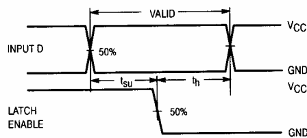
Figure 4. Switching Waveforms
