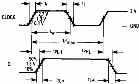
Figure 1. Switching Waveforms
