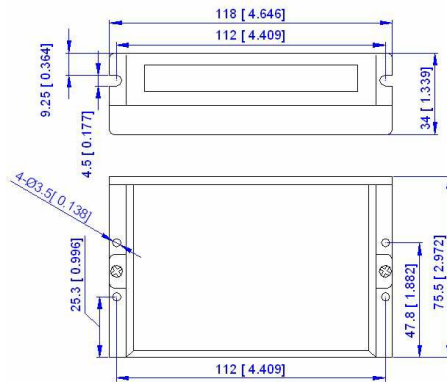
Figure 1: Mechanical specifications
