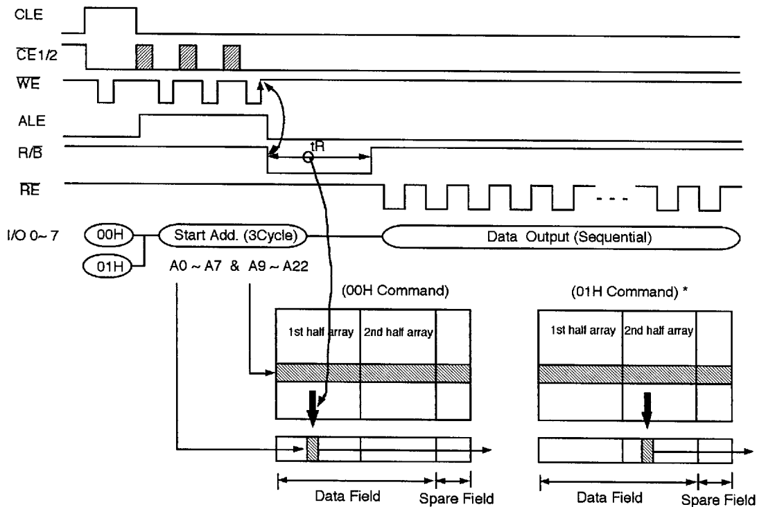
Figure 3. Read 1 Operation
