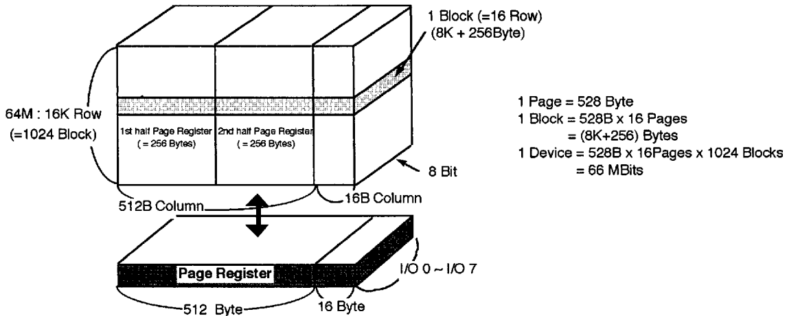
Figure 2. ARRAY ORGANIZATION
