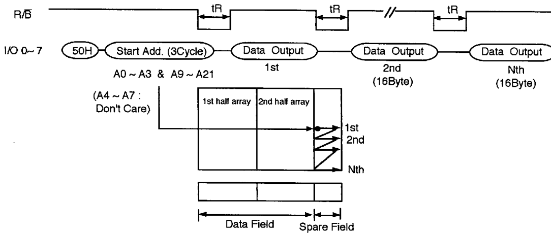
Figure 7. Gap-less Sequential Read Operation ( \overline{SE} = fixed low)
