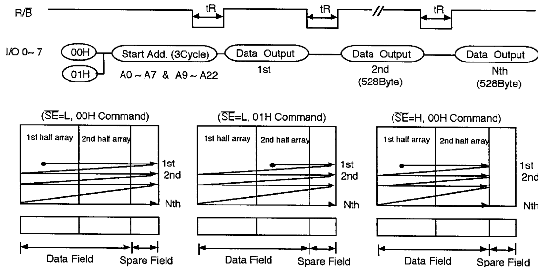
Figure 5. Sequential Row Read 1 Operation
