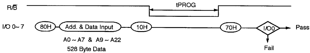
Figure 8. Program & Read Status Operation
