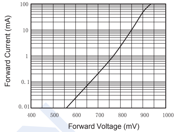
Figure 3. DC Characteristics
