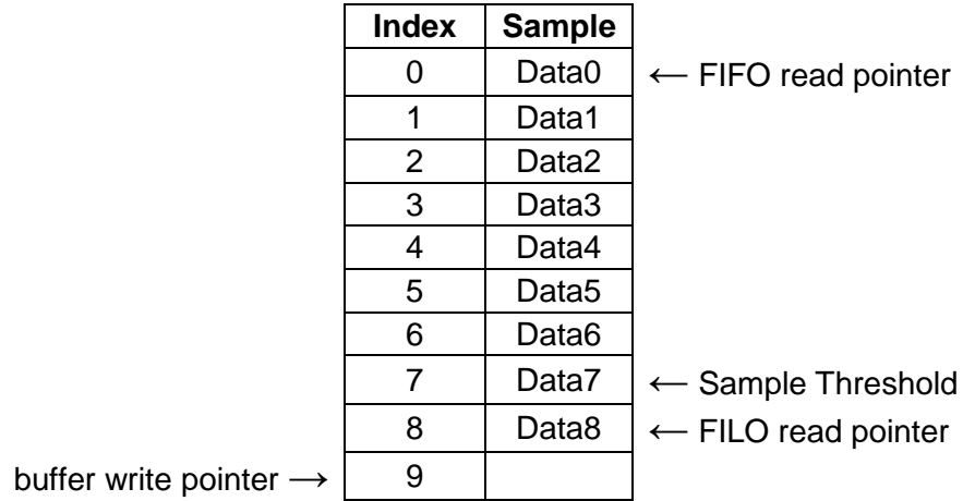
Figure 22. FILO Read from Full Buffer
