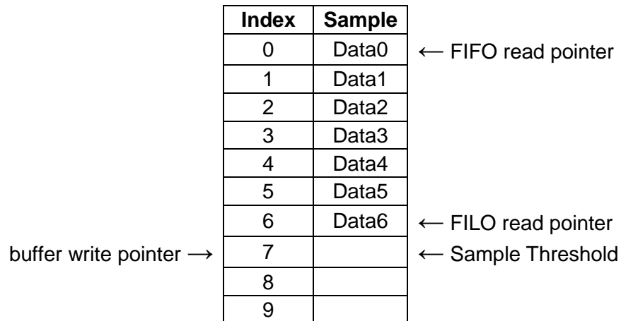
Figure 15. Buffer Approaching Sample Threshold
