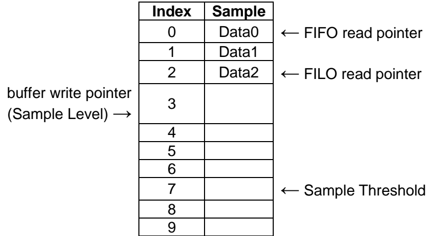
Figure 14. Buffer Filling
