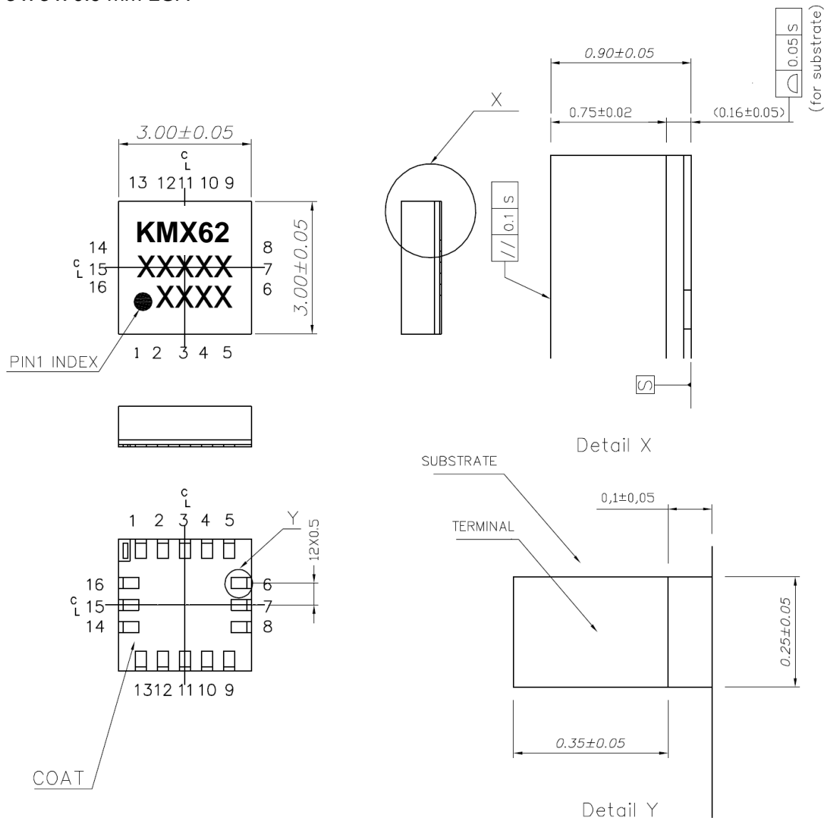
Figure 6. KMX62 Package Dimensions
