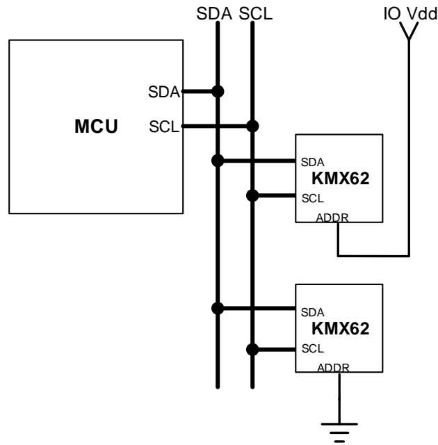
Figure 8. Multiple KMX62 I 2 C Connection
