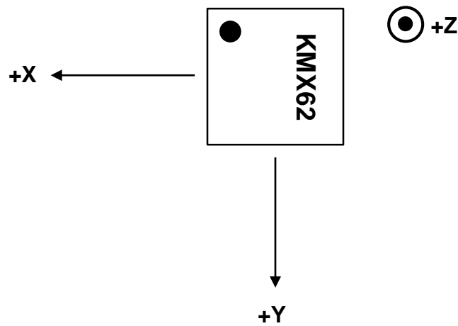
Figure 7. KMX62 Orientation
