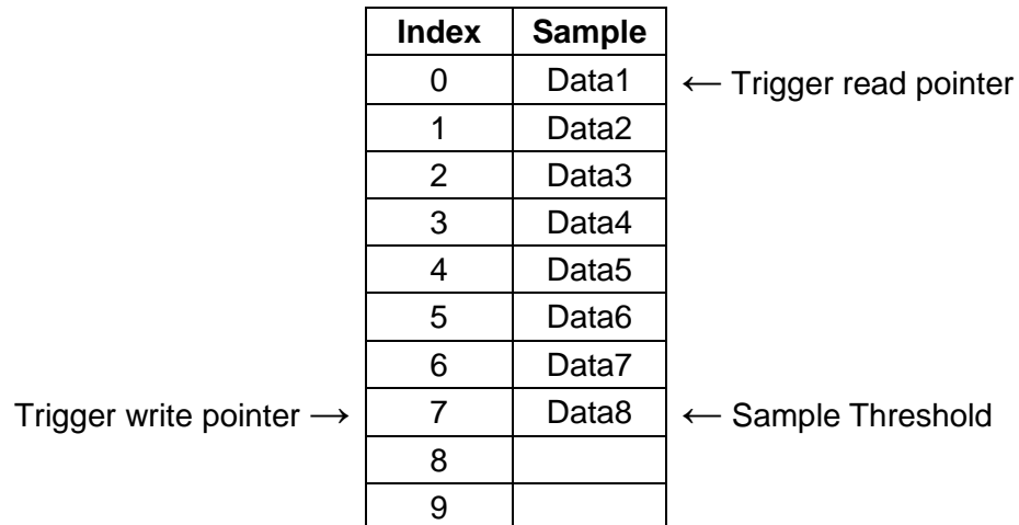
Figure 17. Additional Data Prior to Trigger Event
