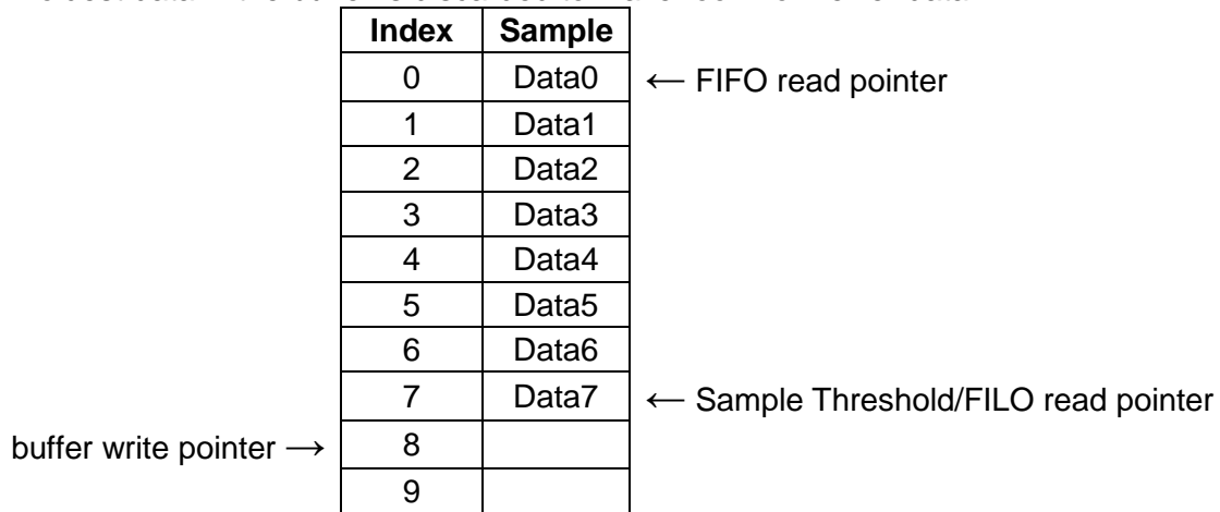
Figure 16. Buffer at Sample Threshold
