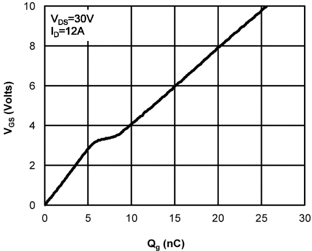
Figure 7: Gate-Charge Characteristics
