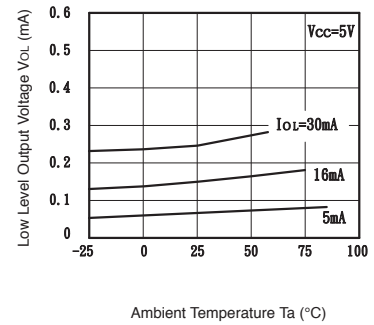
Fig.6 Low Level Output Voltage vs. Ambient Temperature
