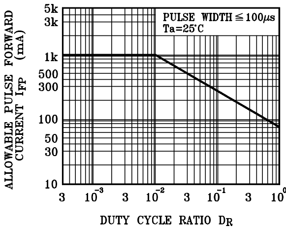
I_{FP} - D_R
