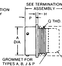
CRIMP KPSE01/MS3121
