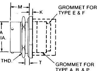
CRIMP KPSE07/MS3124
