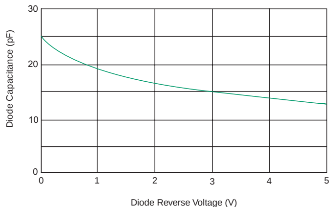
Typical Capacitance vs. Reverse Voltage
