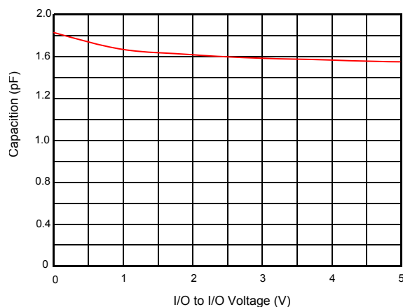
Typical Capacitance vs. Voltage
