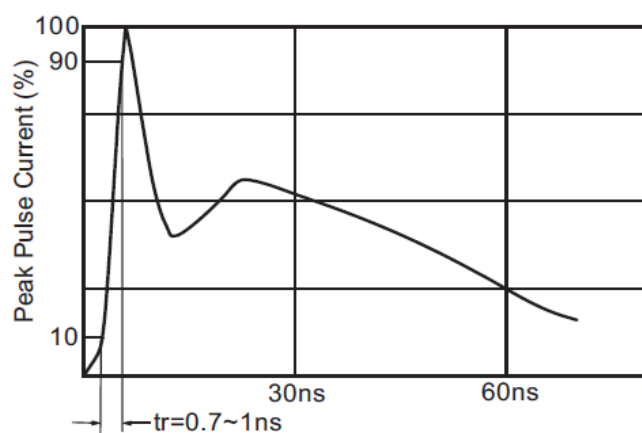
IEC61000-4-2 waveform
