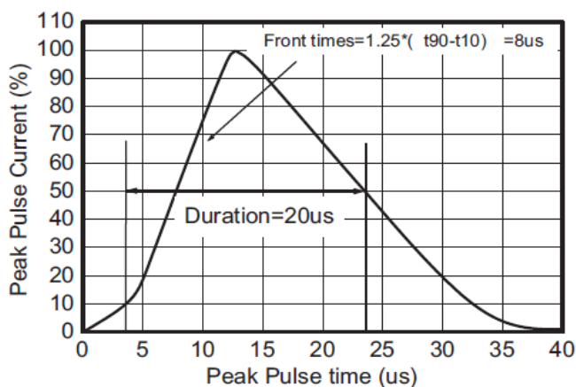
8/20us waveform
