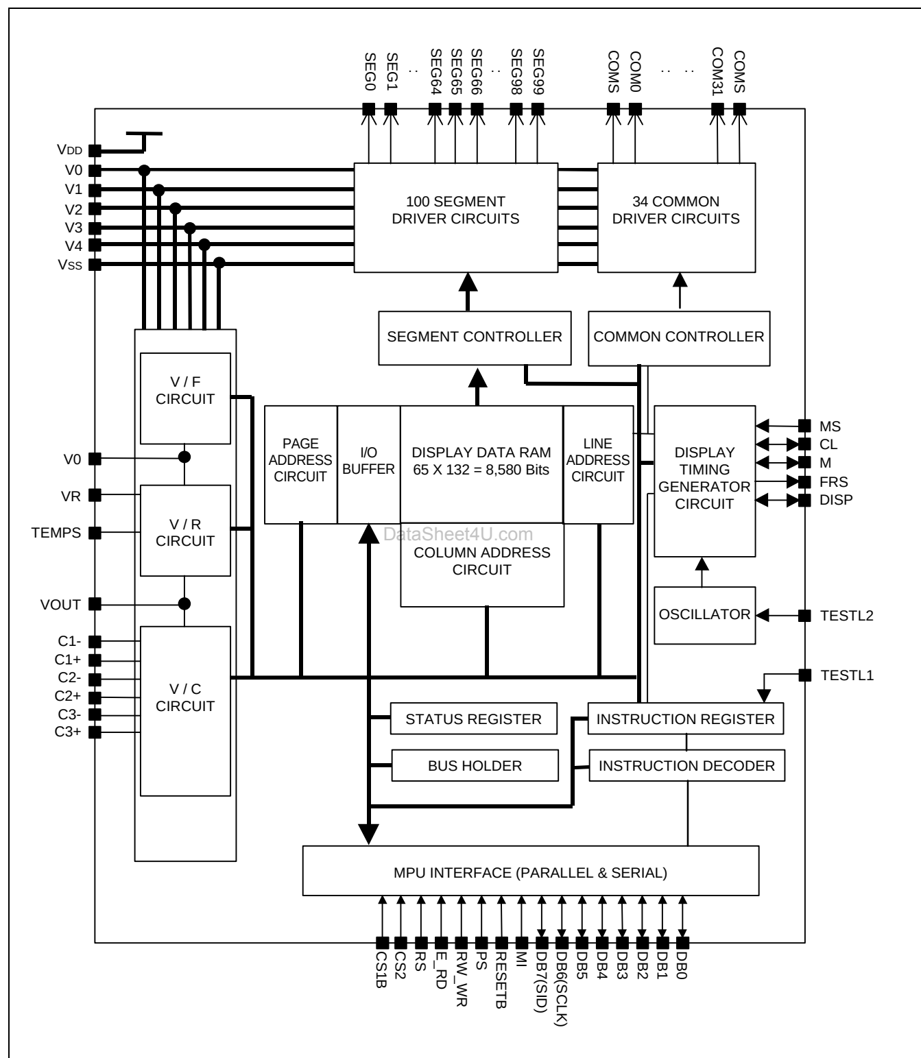
Figure 1. Block Diagram
