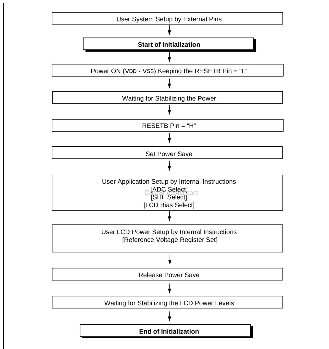
Figure 25. Initializing without the Built-in Power Supply Circuits
