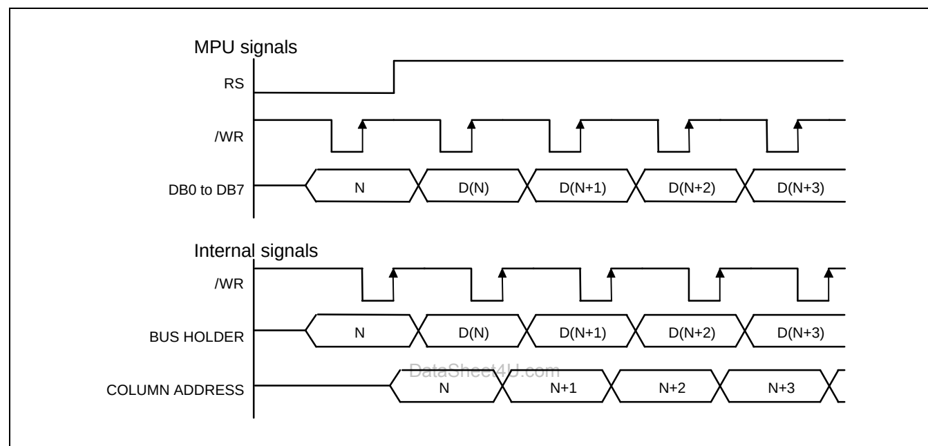
Figure 4. Write Timing
