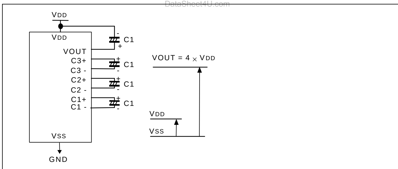
Figure 13. Four Times Boosting Circuit
