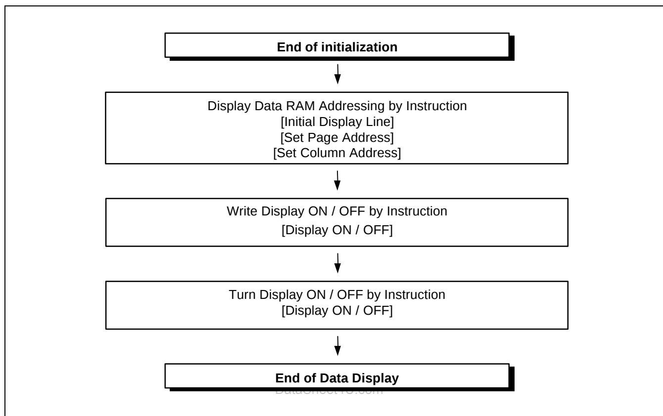
Figure 29. Data Displaying
