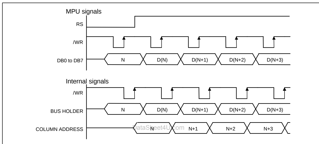
Figure 4. Write Timing
