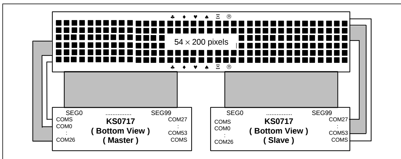
Figure 51. SHL = 1, ADC = 0
