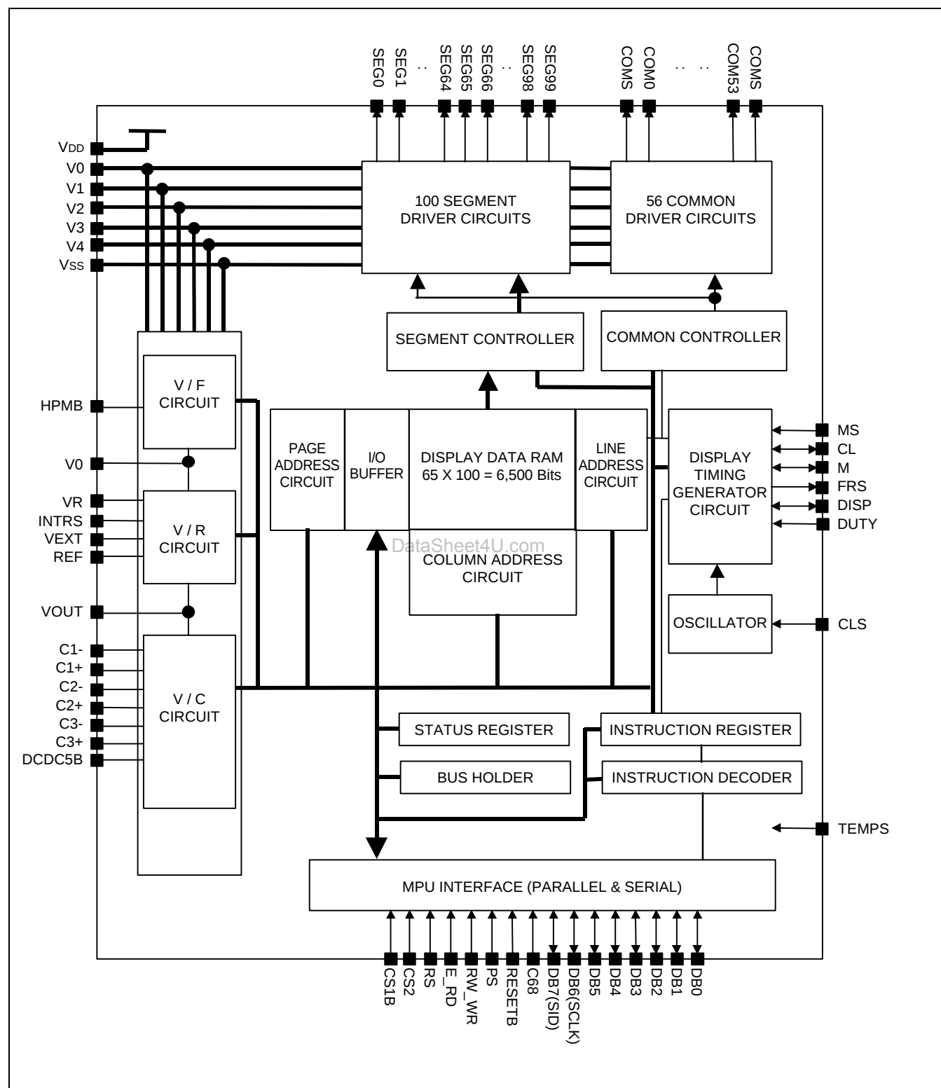
Figure 1. Block Diagram
