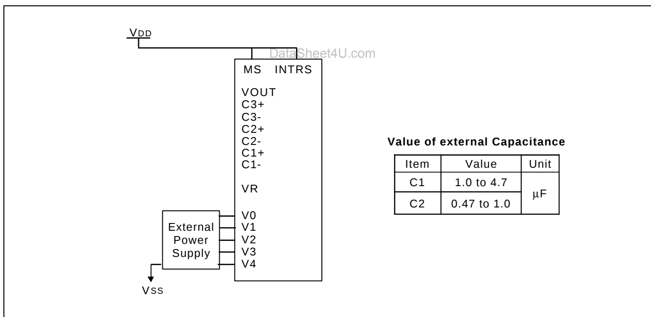
Figure 21. When Not Using any Internal LCD Power Supply Circuits (V/C: OFF, V/R: OFF, V/F: OFF)
