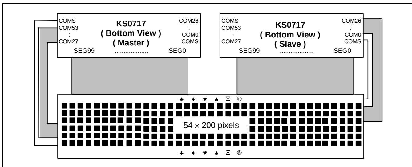
Figure 50. SHL = 0, ADC = 1
