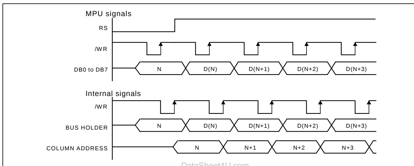
Figure 4. Write Timing
