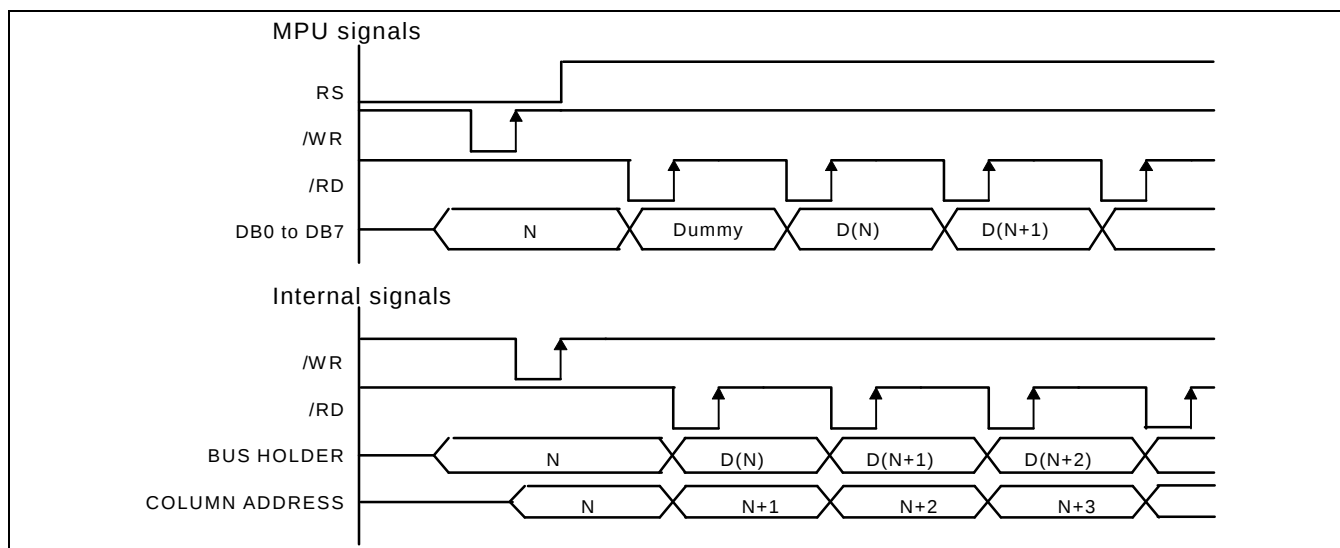
Figure 5. Read Timing
