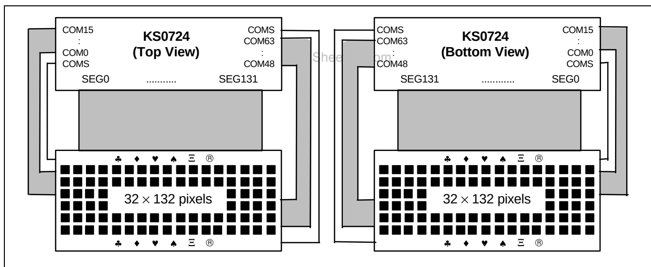
Figure 52. SHL = 0, ADC = 0
