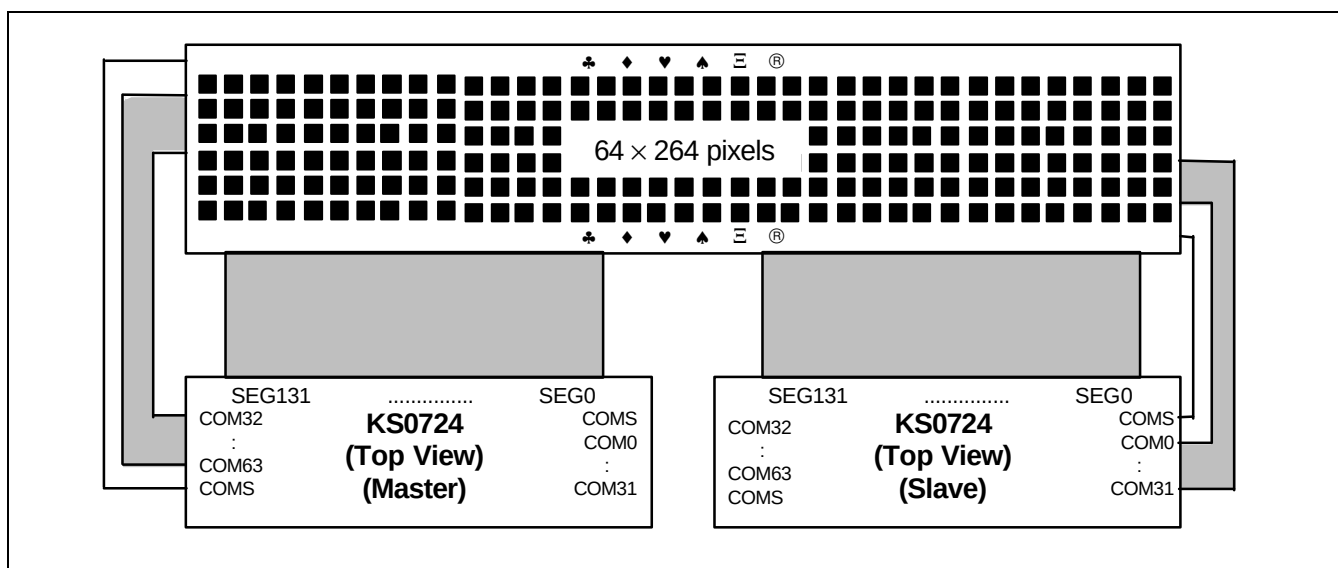
Figure 54. SHL = 1, ADC = 1
