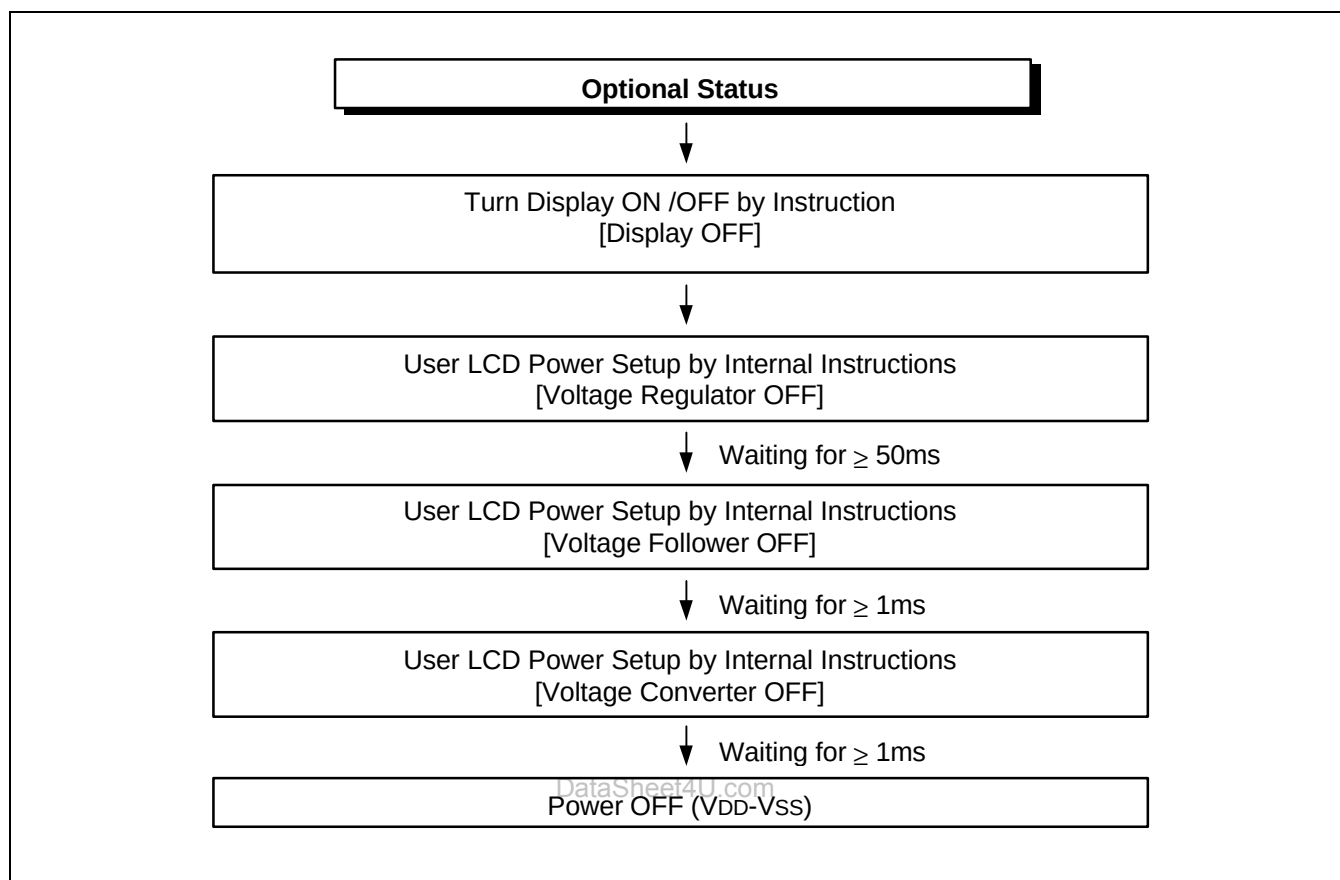
Figure 29. Power OFF
