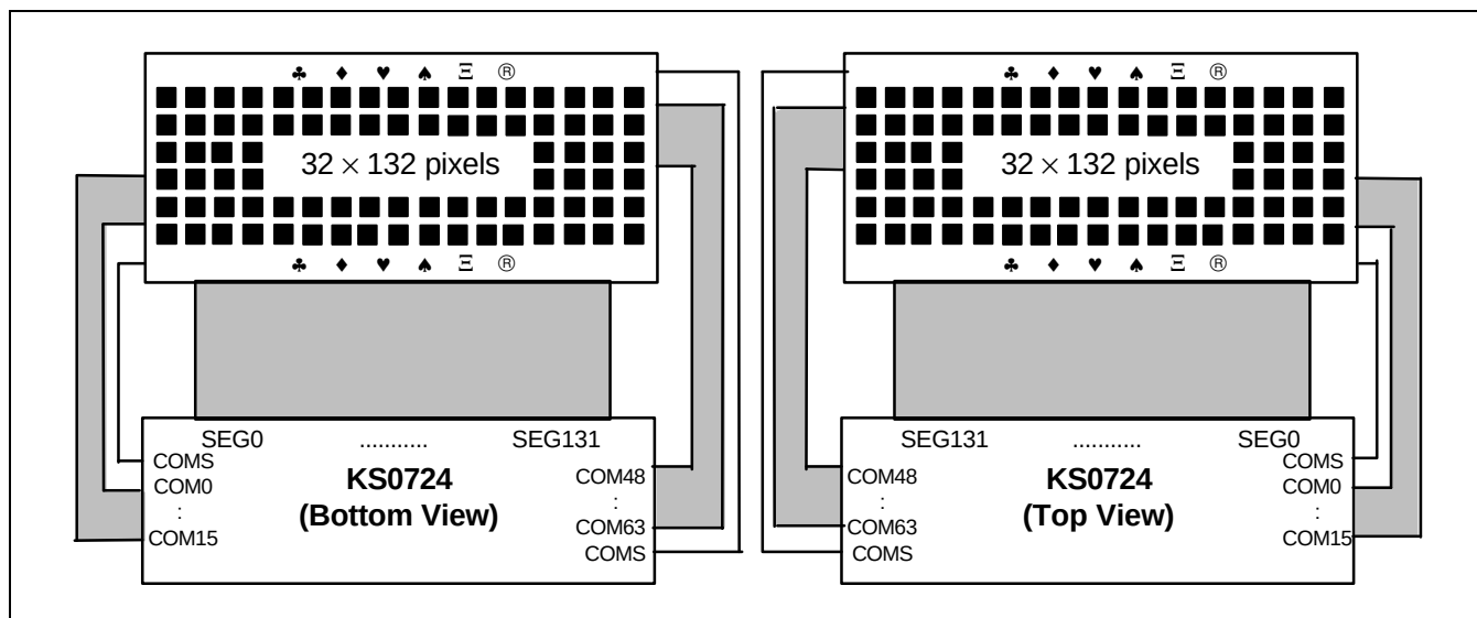
Figure 50. SHL = 1, ADC = 0
