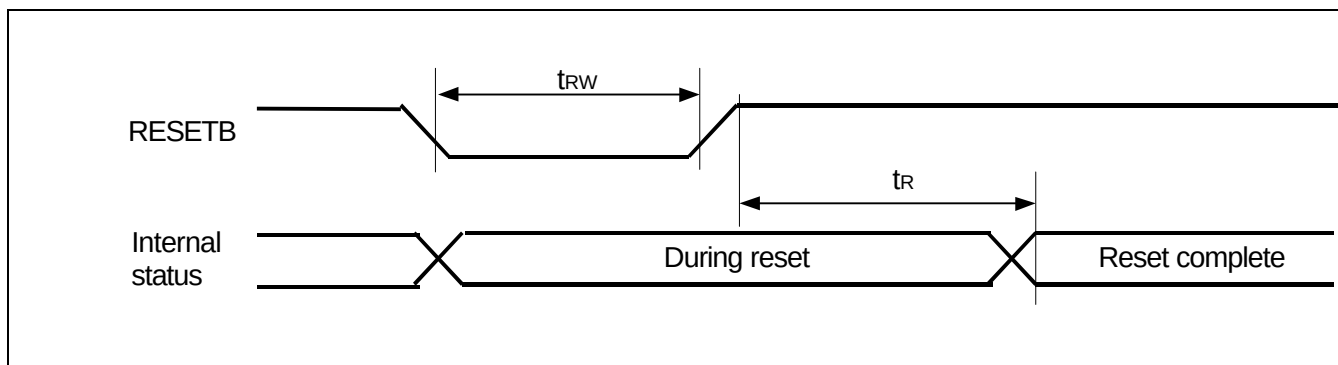
Figure 33. Reset Input Timing
