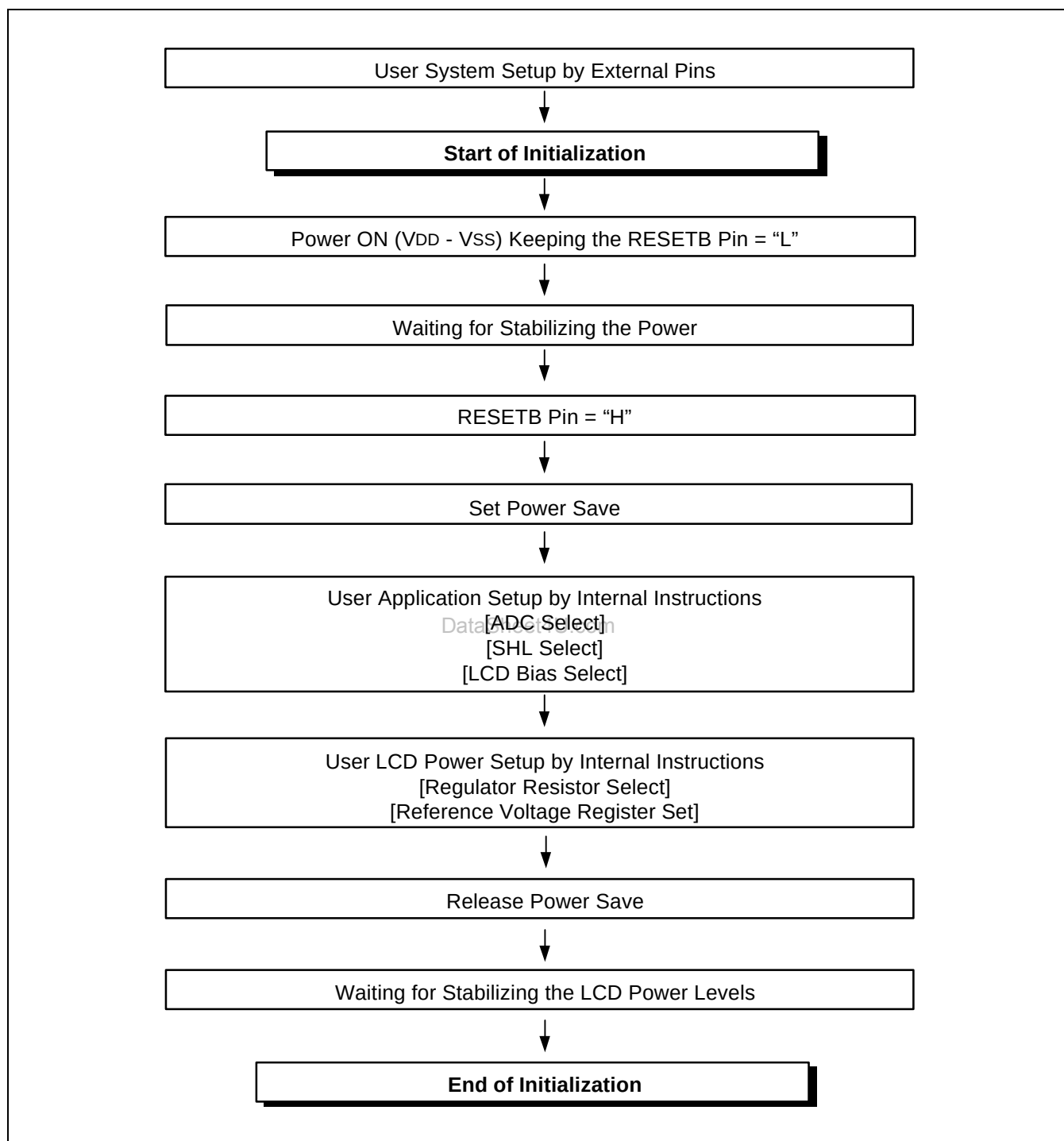
Figure 27. Initializing without the Built-in Power Supply Circuits
