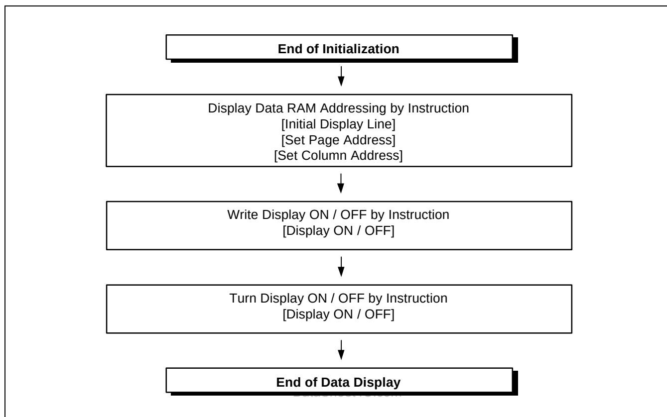
Figure 28. Data Displaying
