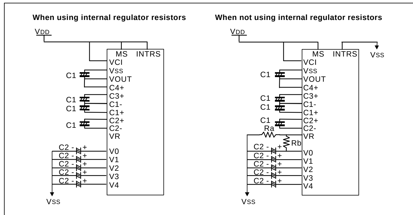
Figure 17. When Using all Internal LCD Power Circuits (VCI = VDD, 4-time VIC: ON, V/R: ON, V/F: ON)
