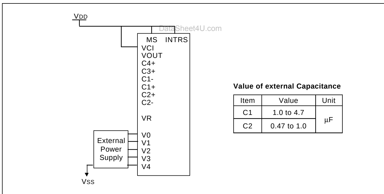
Figure 20. When Not Using any Internal LCD Power Supply Circuits (VCI = VDD, V/I: OFF, V/R: OFF, V/F: OFF)
