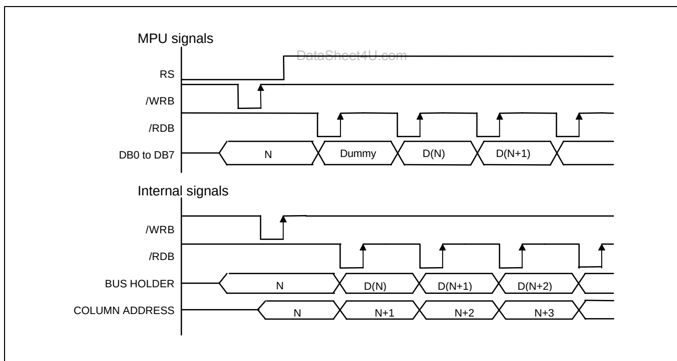
Figure 5. Read Timing
