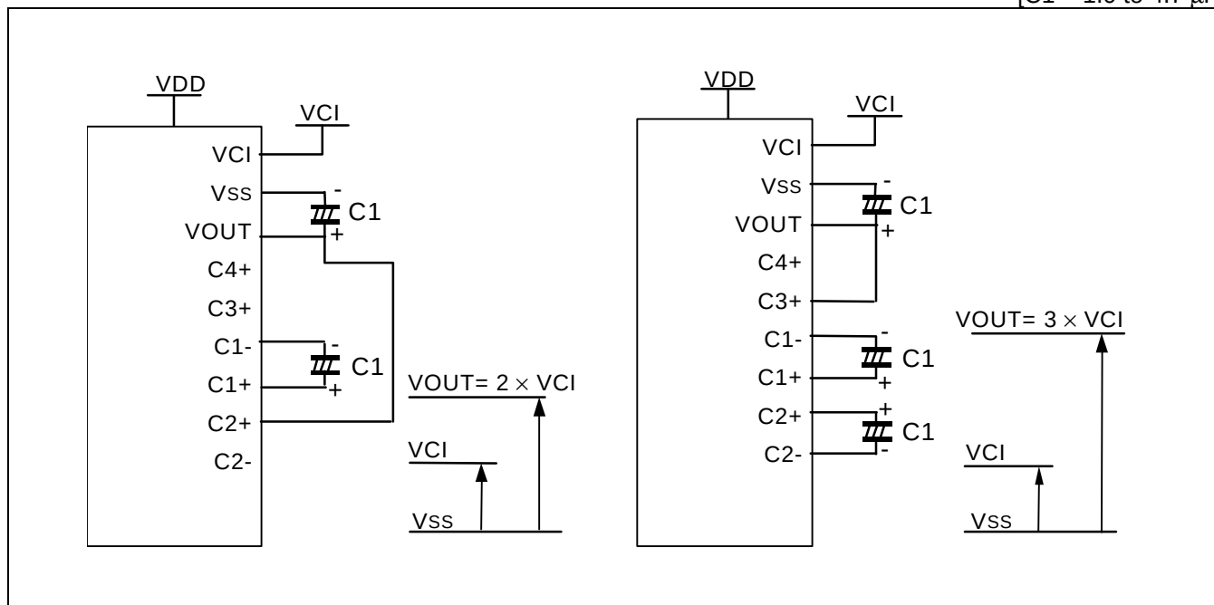
Figure 11. Two Times Boosting Circuit
