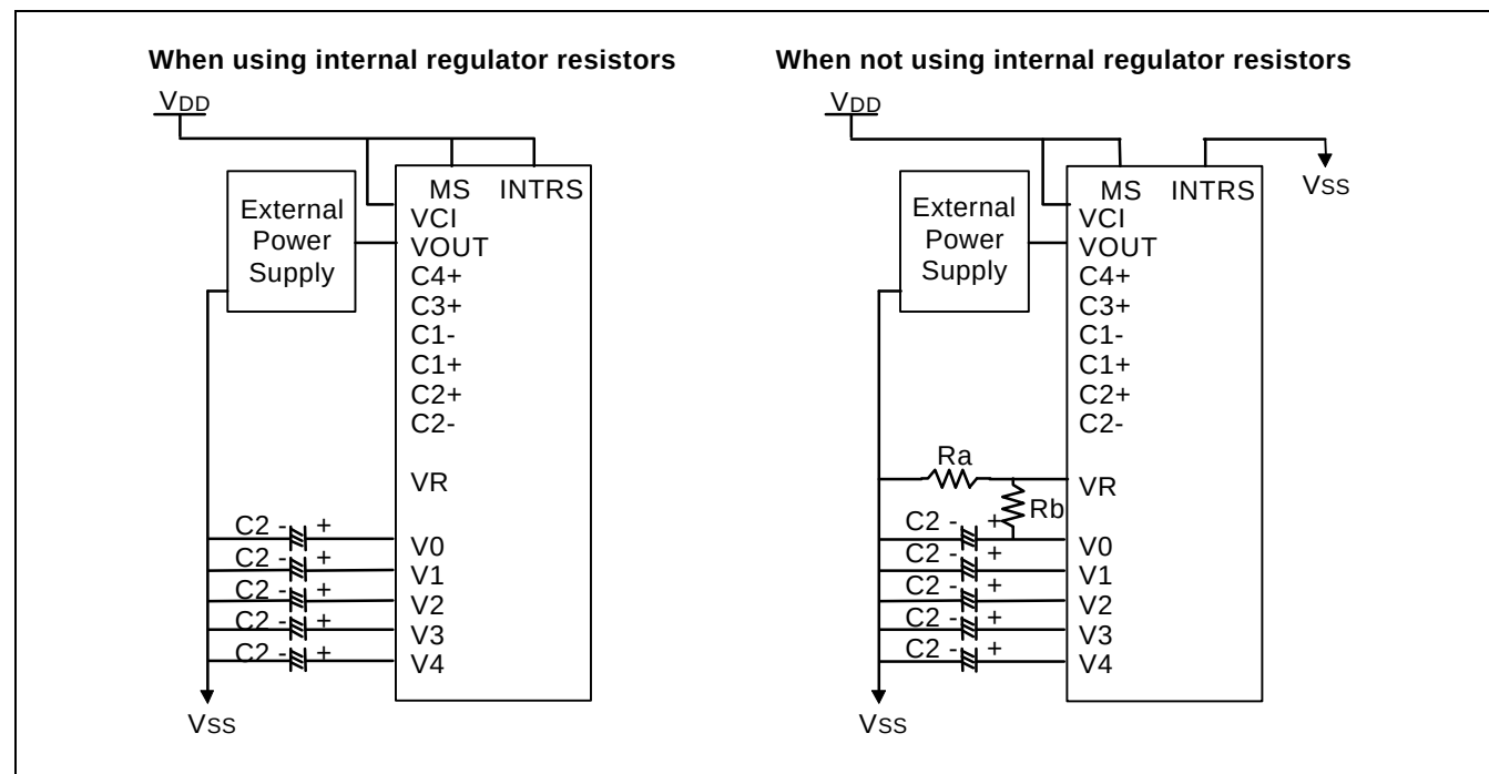
Figure 18. When Using some Internal LCD Power Circuits (VCI = VDD, VIC: OFF, V/R: ON, V/F: ON)
