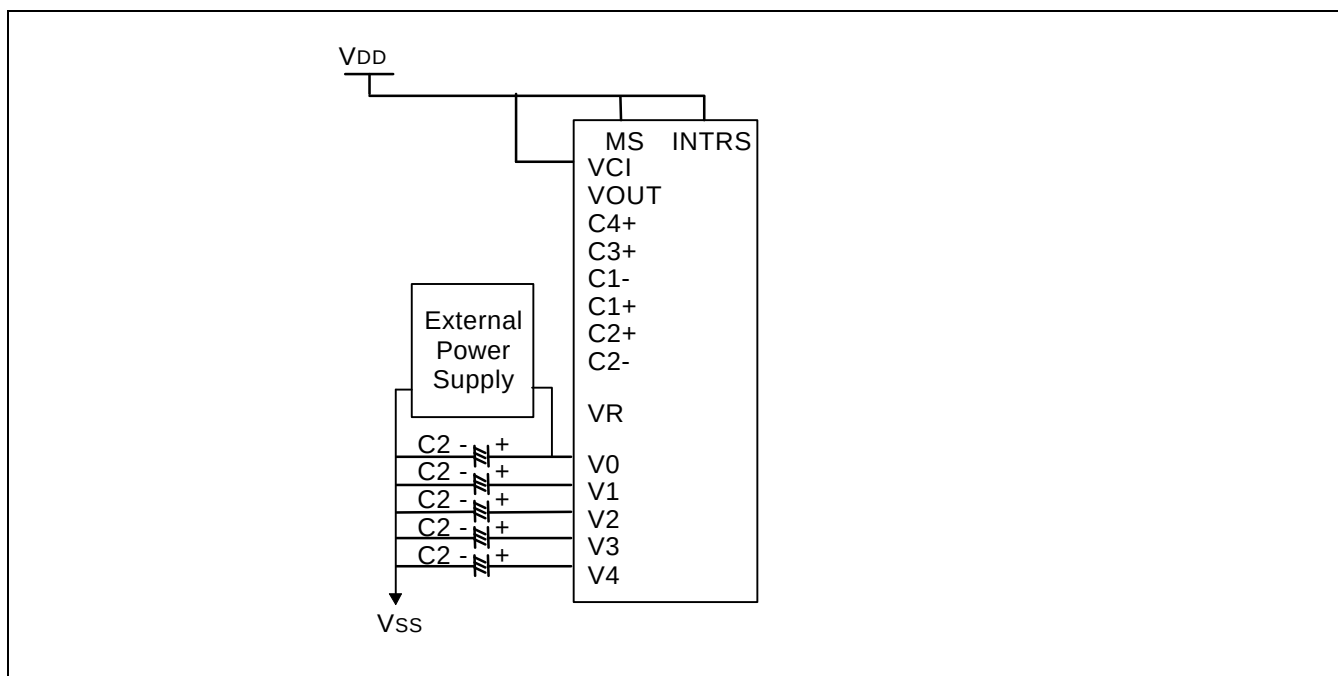
Figure 19. When Using some Internal LCD Power Circuits (VCI = VDD, V/I: OFF, V/R: OFF, V/F: ON)
