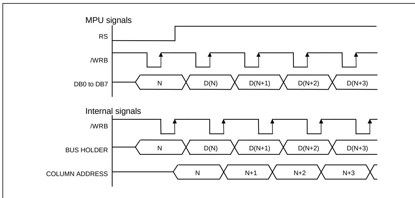
Figure 4. Write Timing
