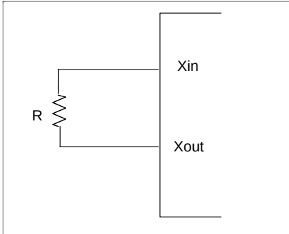
Figure 19. RC Oscillator (only for the KS57C0002)
