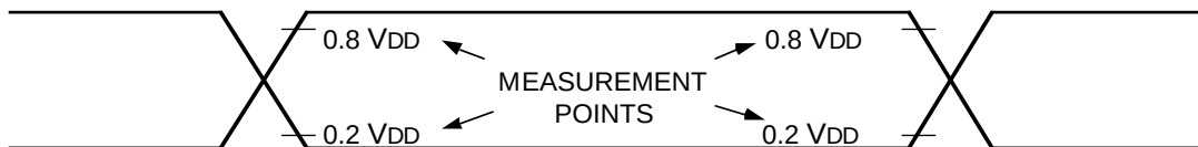
Figure 37. A.C. Timing Measurement Points (Except for X in )
