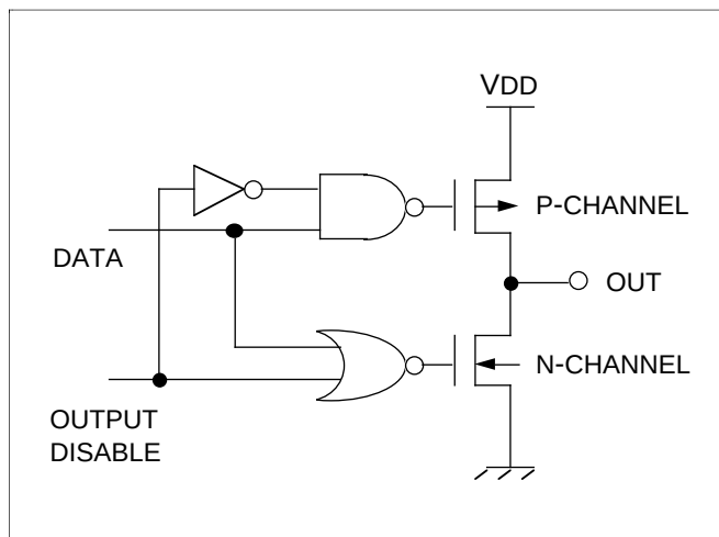
Figure 6. Pin Circuit Type 4
