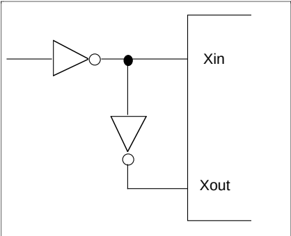
Figure 18. External Clock
