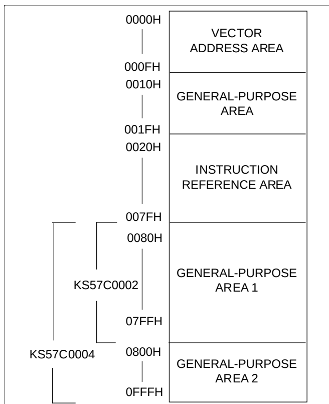
Figure 12. ROM Map
