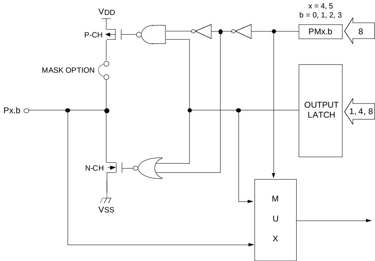
Figure 25. Circuit Diagram for Ports 4 and 5
