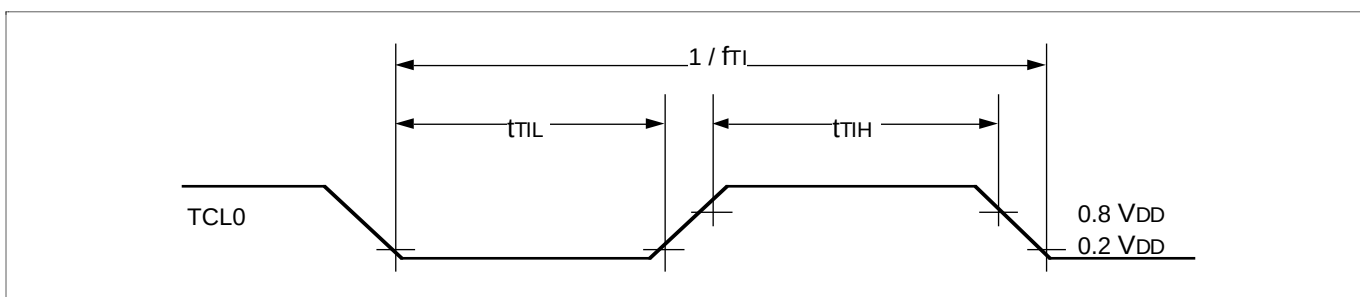
Figure 41. TCL0 Timing
