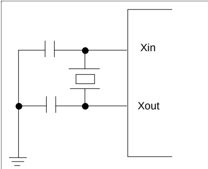
Figure 17. Crystal/Ceramic Oscillator
