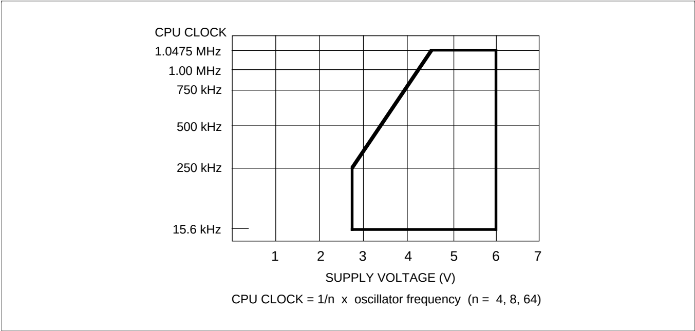
Figure 36. Standard Operating Voltage Range
