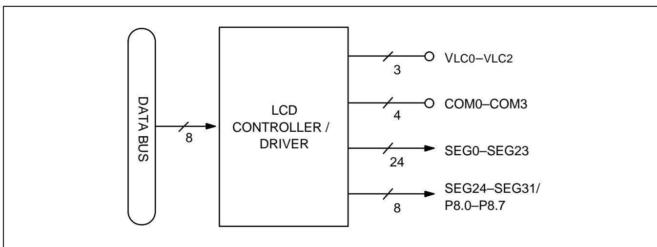
Figure 12-1. LCD Function Diagram
