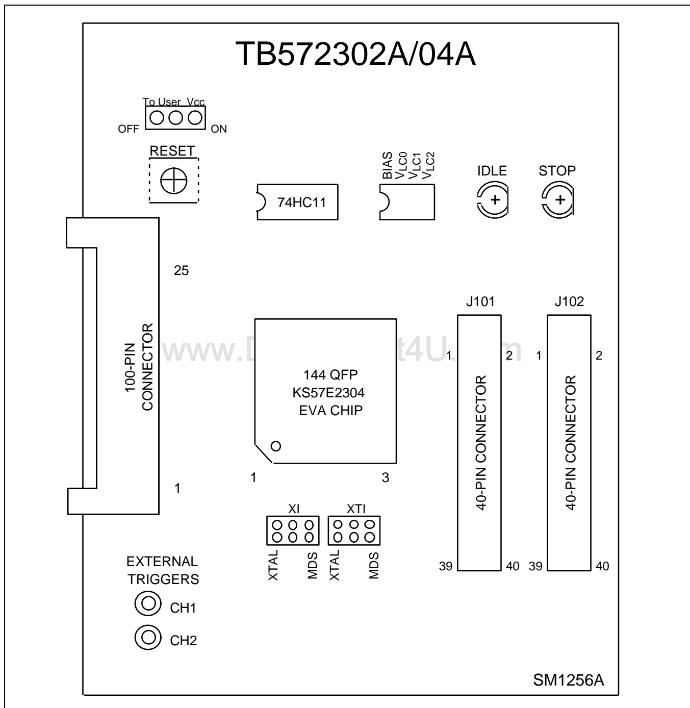
Figure 16-2. TB572302A/04A Target Board Configuration
