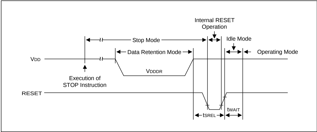
Figure 18-3. Stop Mode Release Timing When Initiated by RESET
