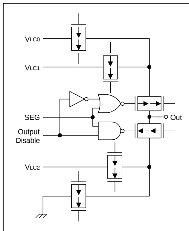
Figure 1-15. Pin Circuit Type H-4
