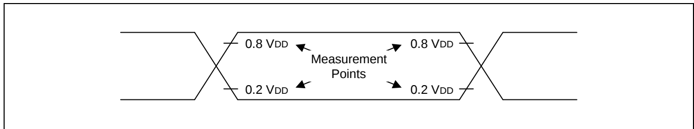
Figure 18-5. A.C. Timing Measurement Points (Except for X_{IN} and XT_{IN} )
