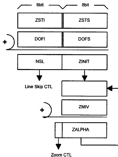
Fig. 1 Relation of Zoom Reg. &amp; DIS Reg.
