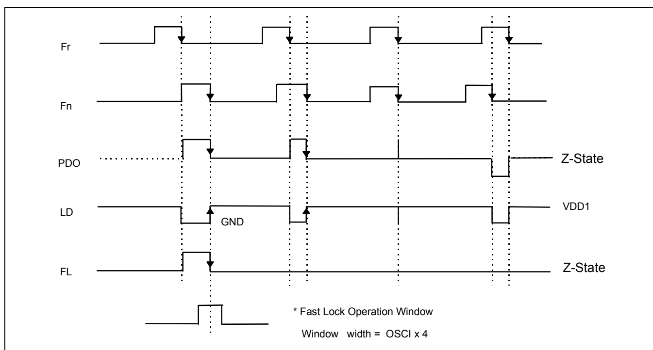
Figure 6. Figure 5-2. Phase Detector / Lock Detector / Fast Lock Output Waveforms
