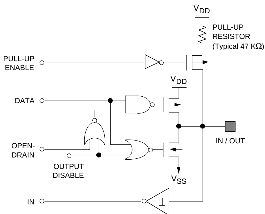
Figure 4. Pin Circuit Type 1 (Ports 0, 1, and 5)
