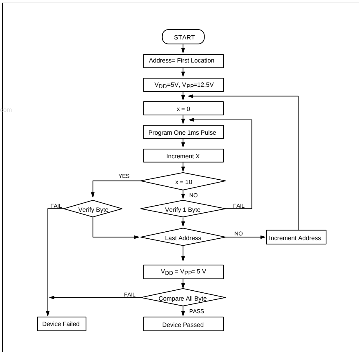
Figure 16-3. OTP Programming Algorithm
