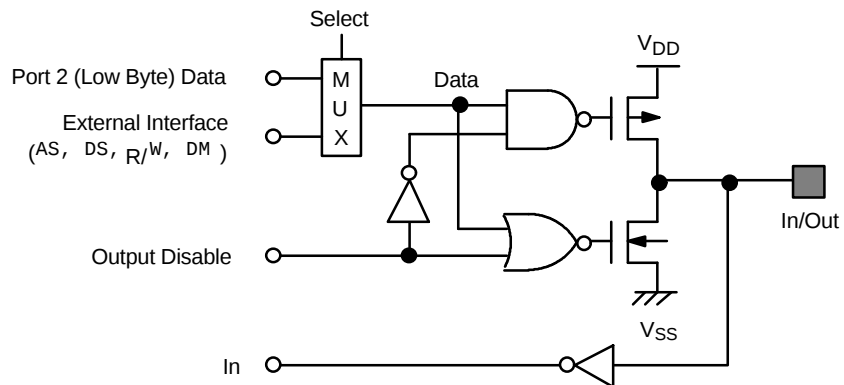
Figure 1-6. Pin Circuit Type D-1 (P2.0-P2.3)
