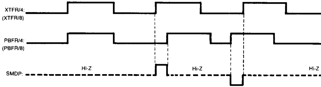
Fig. 19 The timing chart of SMDP output
