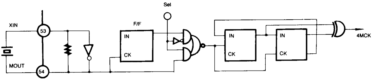
Fig. 6 X'tal OSC Block Diagram
