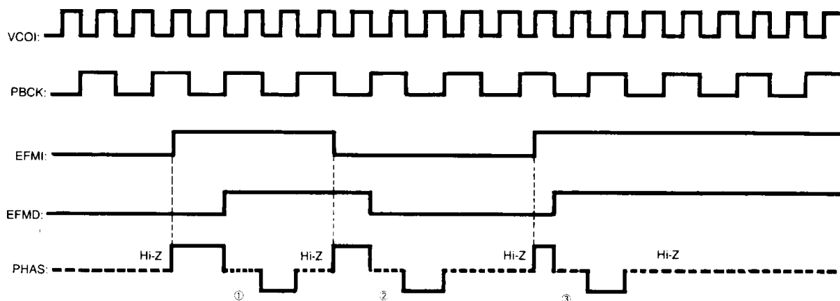
Fig. 7 EFM Phase Detection Timing Chart
