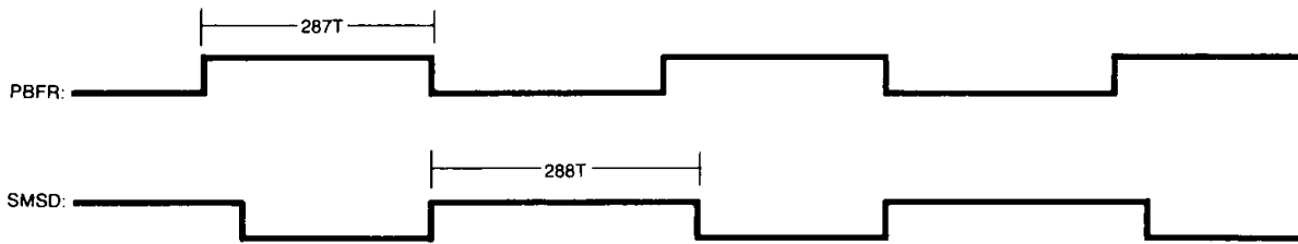
(a) The timing chart of SMSD output when PBFR is '287T'
