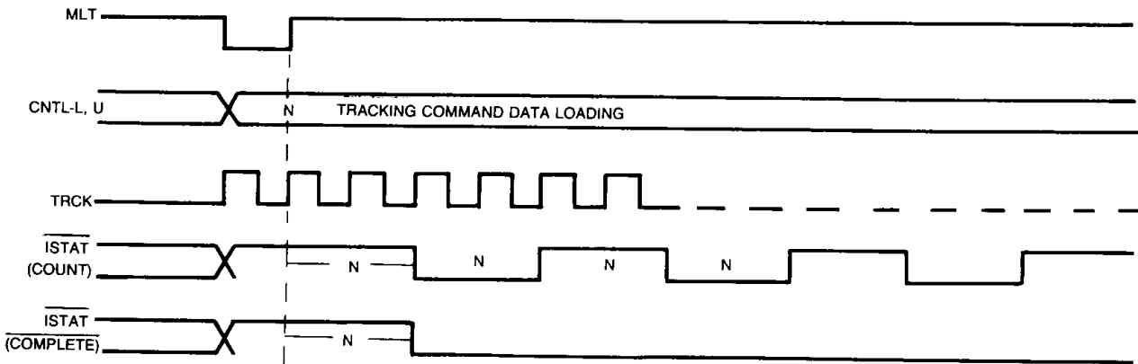
Fig. 4 Tracking Count Timing Chart
