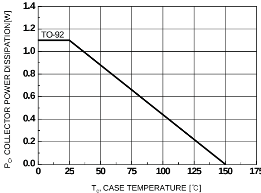
Figure 6. Power Derating
