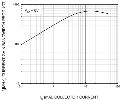
Figure 5. f_T - I_C
