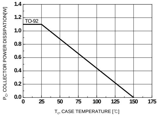
Figure 6. Power Derating
