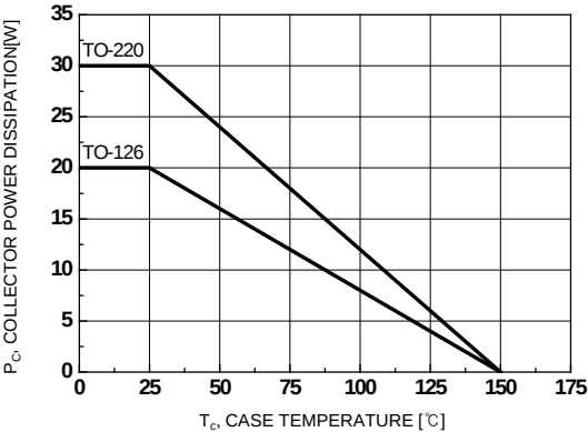
Figure 8. Power Derating
