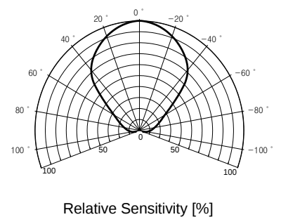
Radiant pattern
