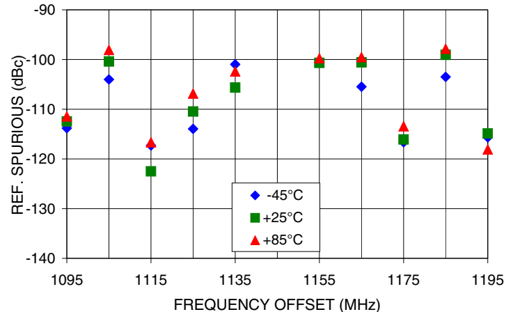
REFERENCE SPURIOUS Vs FREQ. OFFSET @ Fcar = 1145MHz
