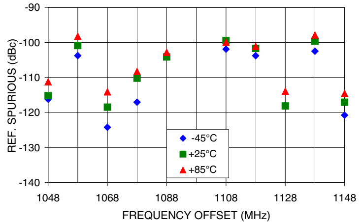
REFERENCE SPURIOUS Vs FREQ. OFFSET @ Fcar = 1098MHz
