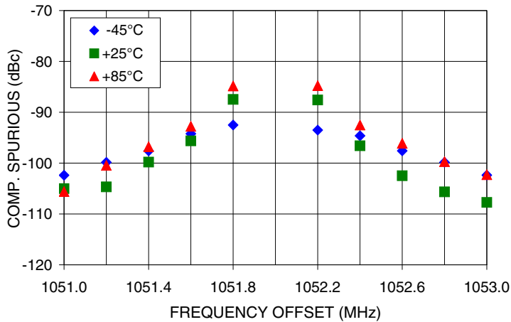
COMPARISON SPURIOUS Vs FREQ. OFFSET @ Fcar = 1052MHz
