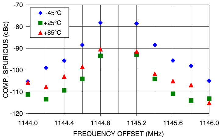
COMPARISON SPURIOUS Vs FREQ. OFFSET @ Fcar = 1145MHz
