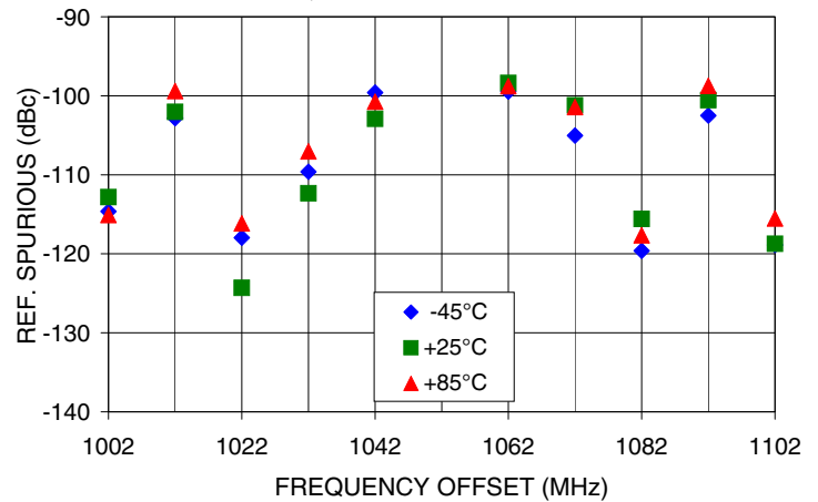
REFERENCE SPURIOUS Vs FREQ. OFFSET @ Fcar = 1052MHz
