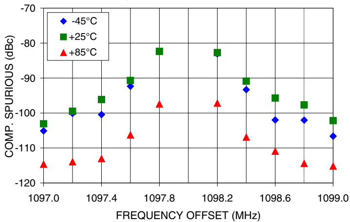
COMPARISON SPURIOUS Vs FREQ. OFFSET @ Fcar = 1098MHz
