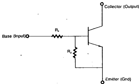
Equivalent Circuit
