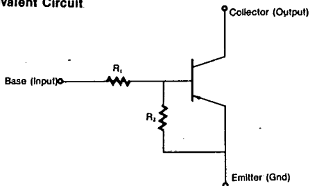
Equivalent Circuit
