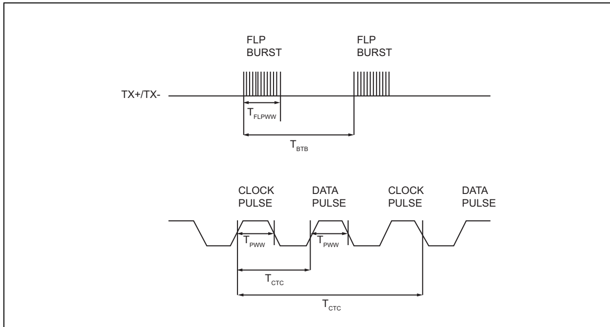
FIGURE 7-2: AUTO-NEGOTIATION TIMING
