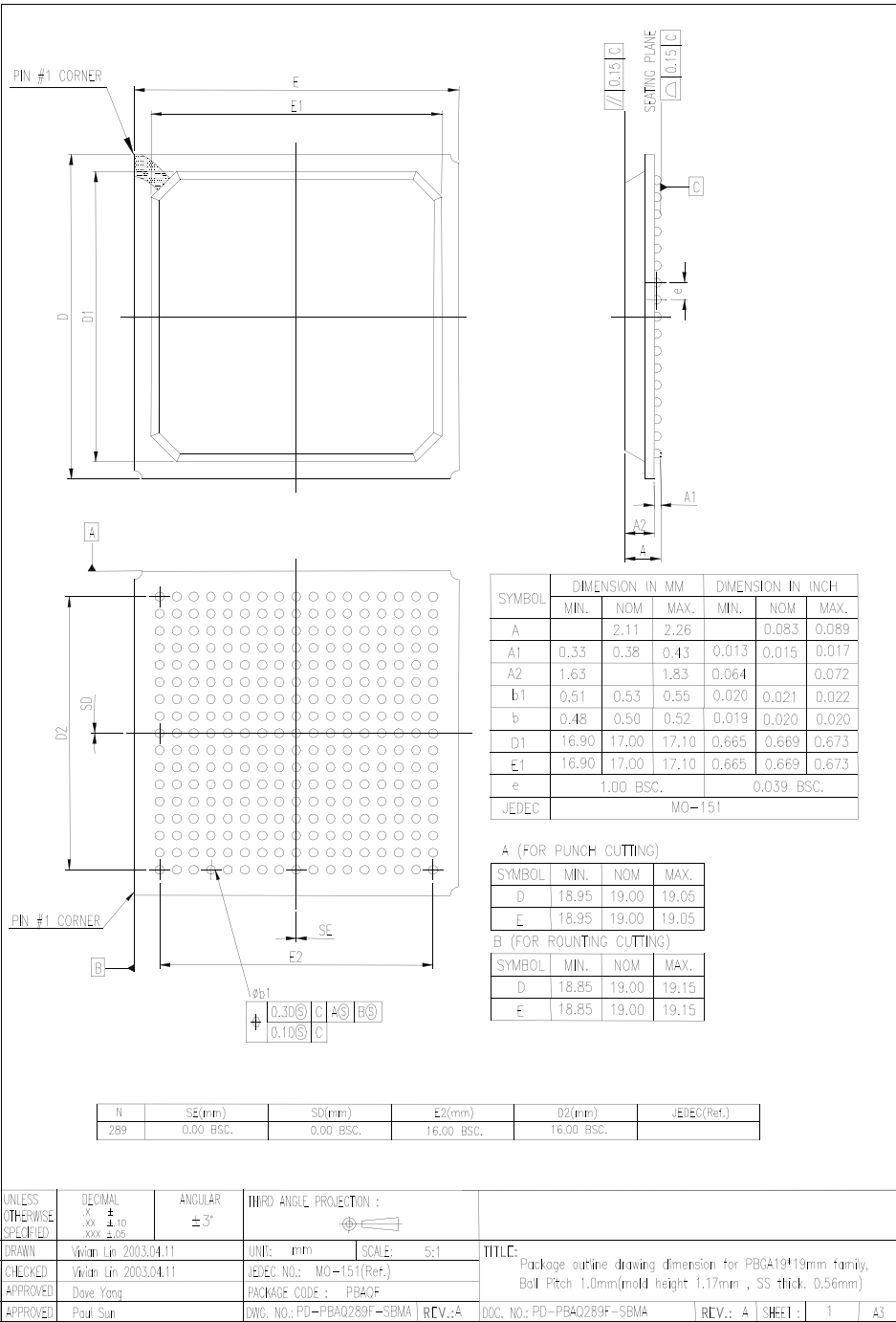
289-Pin PBGA
