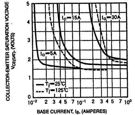
COLLECTOR-EMITTER SATURATION VOLTAGE (TYPICAL)
