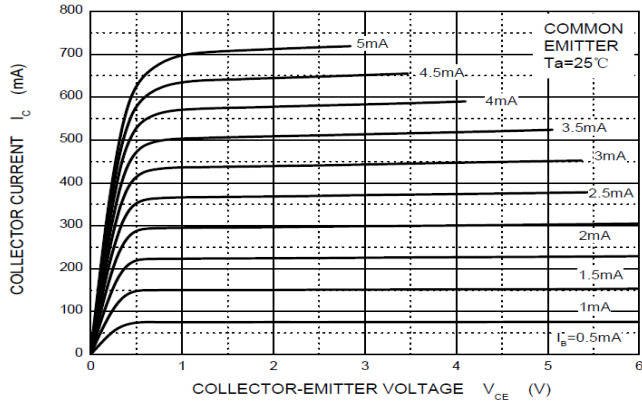
Static Characteristic
