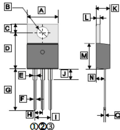
TO-220J
