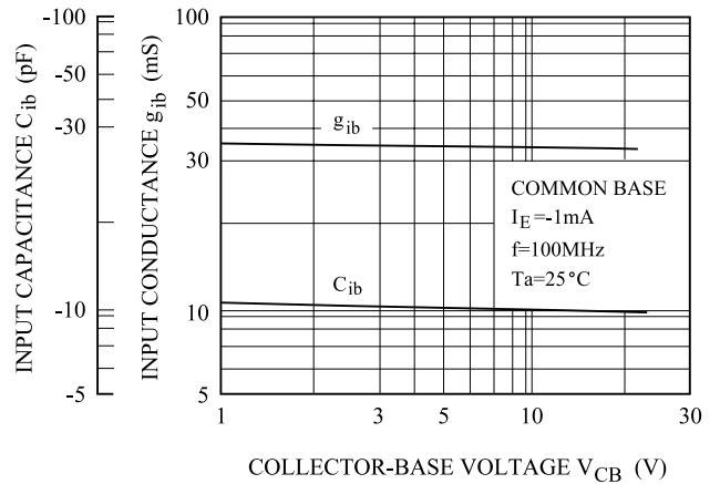
C_{ib}, g_{ib} - V_{CB}
