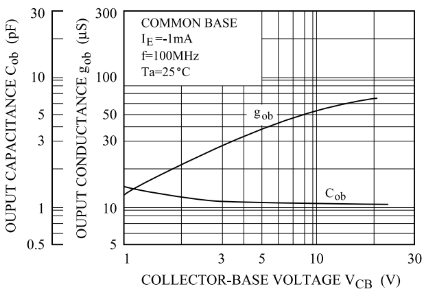
C_{ob}, g_{ob} - V_{CB}
