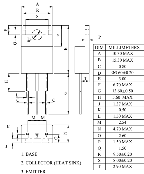
TO-220AB
