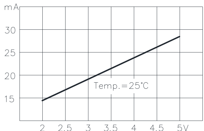
VOLTAGE-CURRENT CONSUMPTION
