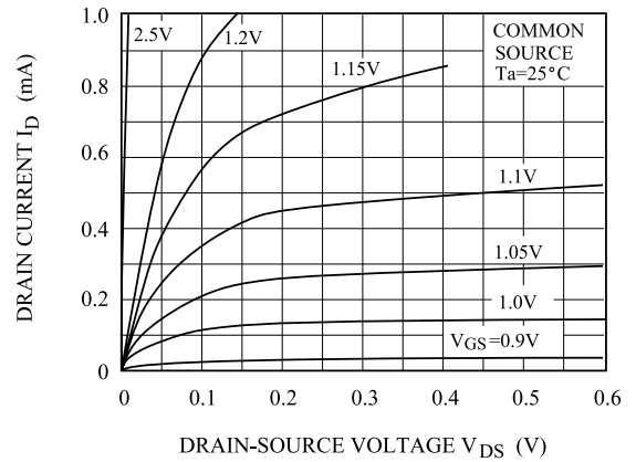
I_D - V_{DS} (LOW VOLTAGE REGION)
